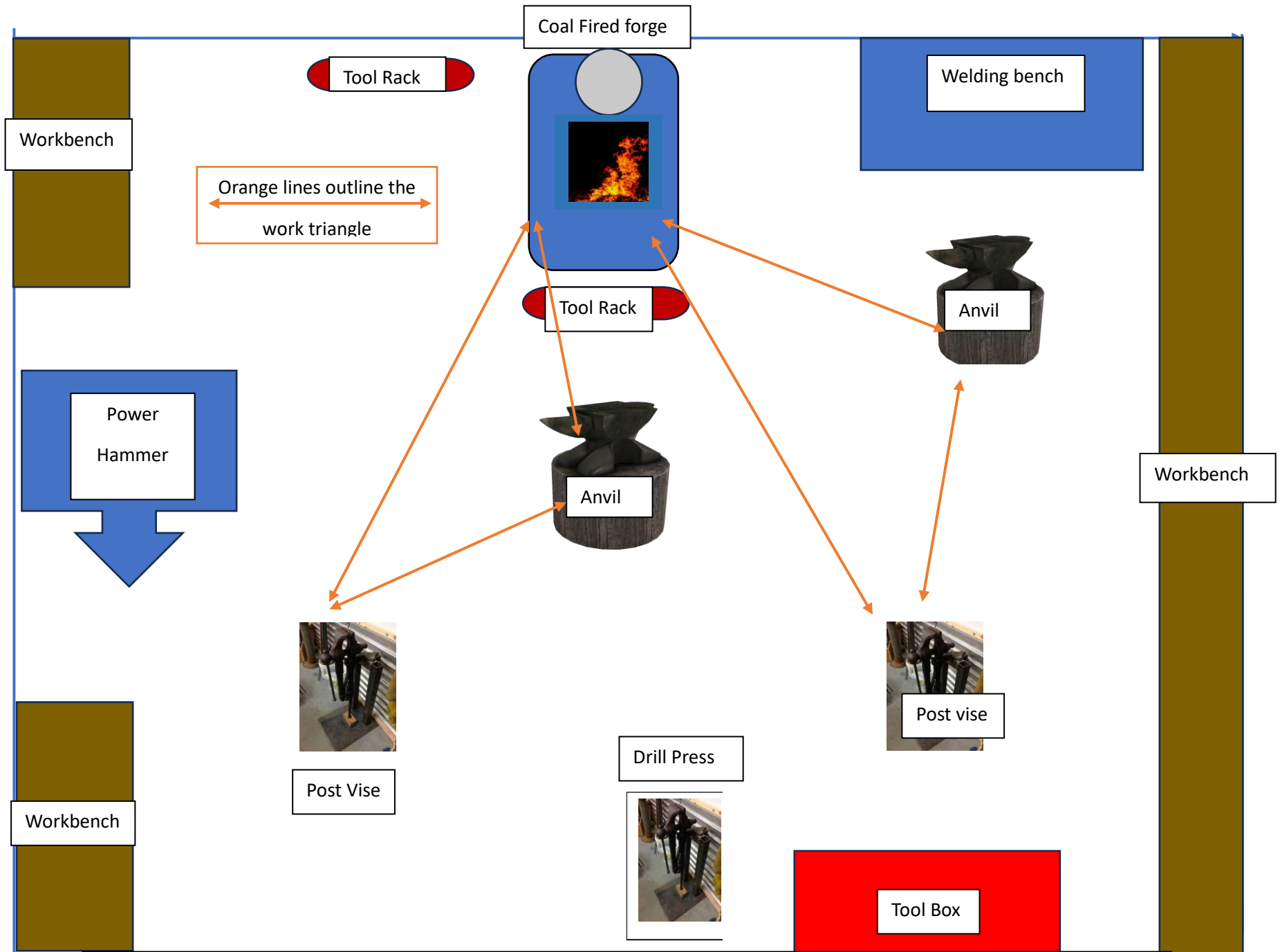
General layout of Jeep's Forge main shop. The shop is 14' wide X 24' long.
